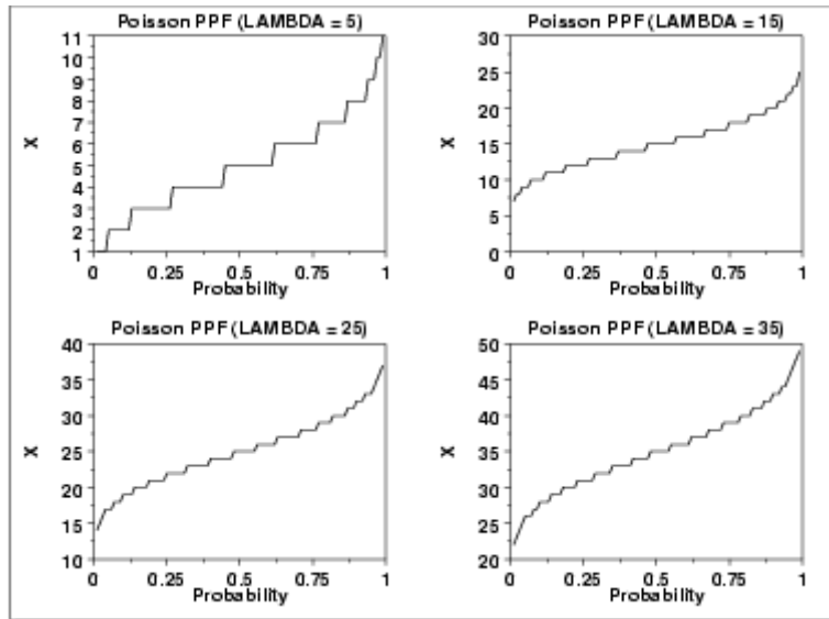
Figure 1: Poisson Distribution for Volume with Different Lambda
