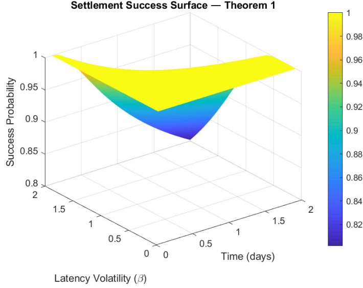
Figure 2: Settlement success surface as a function of latency volatility \beta and time t .
