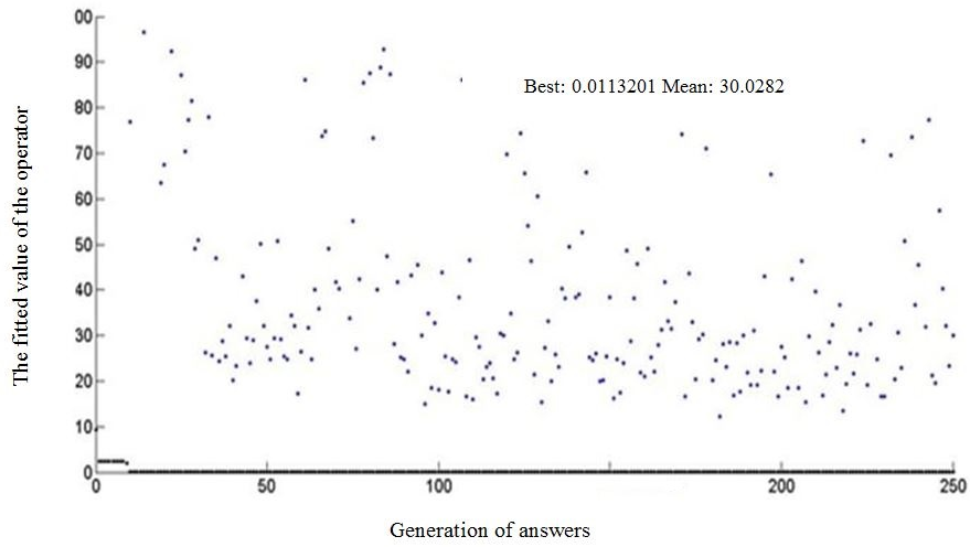
Figure 1: The change trend of Tournament operator in each generation of the simulation (researcher's findings)
