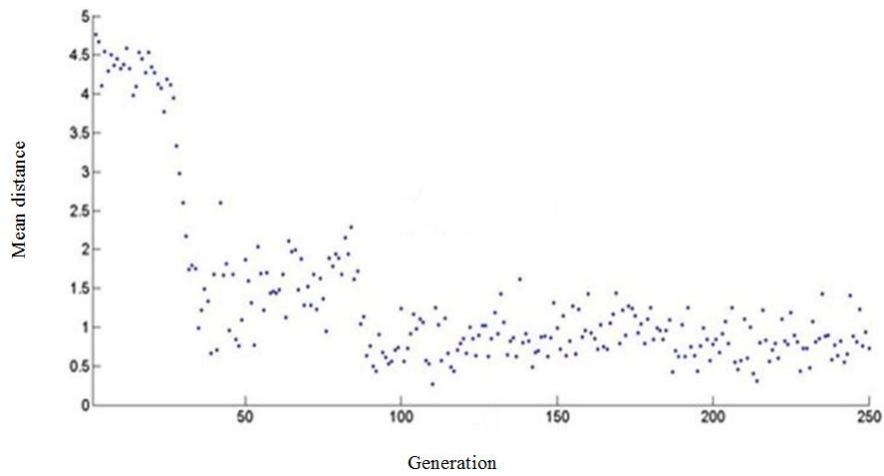
Figure 2: The distance between each generation of Tournament's operator (researcher's findings)
