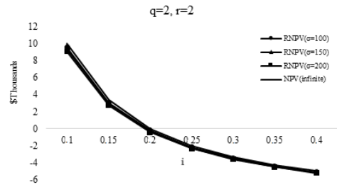
Figure 3: Comparison of different R\hat{N}PV s with different \sigma_{max} when q = 2
