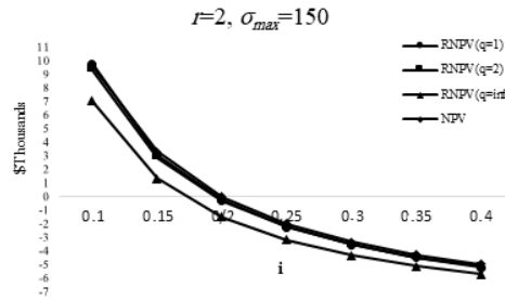
Figure 8: Comparison of different R\hat{N}PV s for different norms
