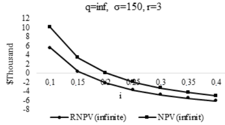
Figure 1: Comparison of R\hat{NPV} and NPV
