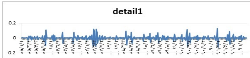
Figure 2: Second level smooth serie (the general trend - STEH1's return
